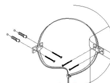
I处放大图 Enlarged view at I
